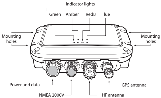
Figure 2 AIS transceiver overview
