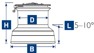
Dimensions Diagram Grand Prix Racing Winch
