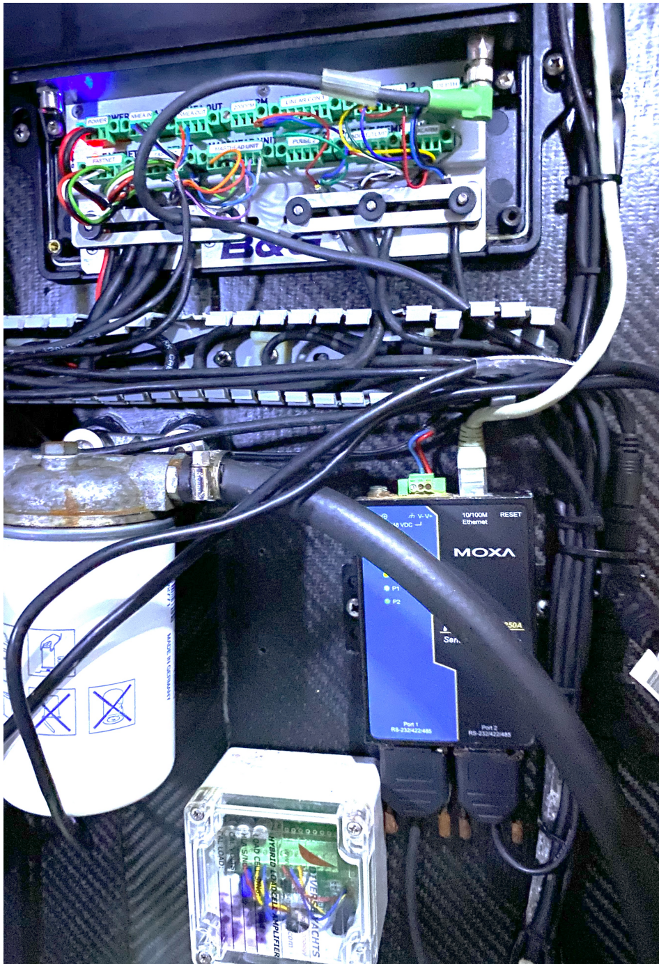
MOXA NPORT SERIAL DEVICE SERVER CONNECTIONS
